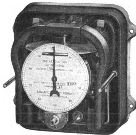
SANGAMO AMPERE HOUR ELECTRIC METER.
